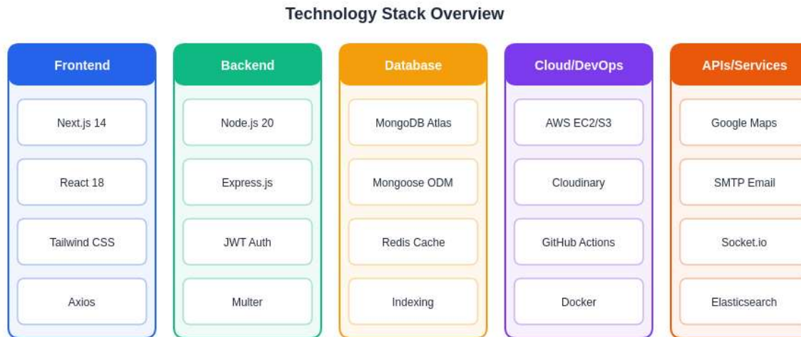
Fig. 5. Technology stack overview showing component distribution across layers
