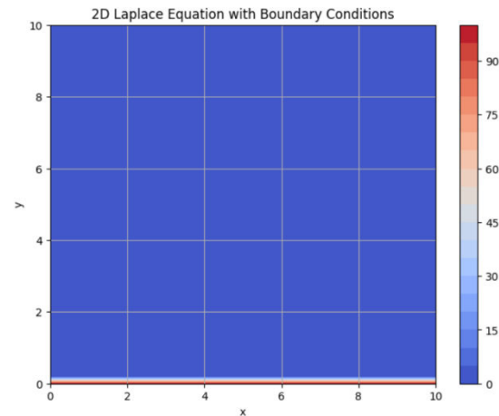
Fig 1 : 2D Laplace Equation With Boundary Conditions
